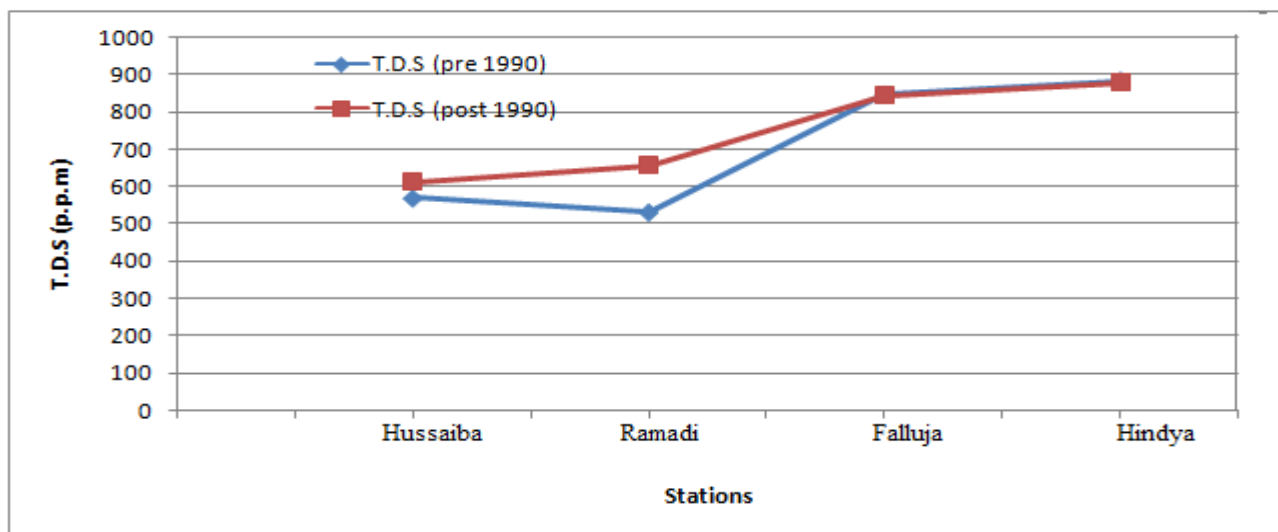
Fig. 15 Salinity along Euphrates River Pre. and post 1990. (Researchers)
