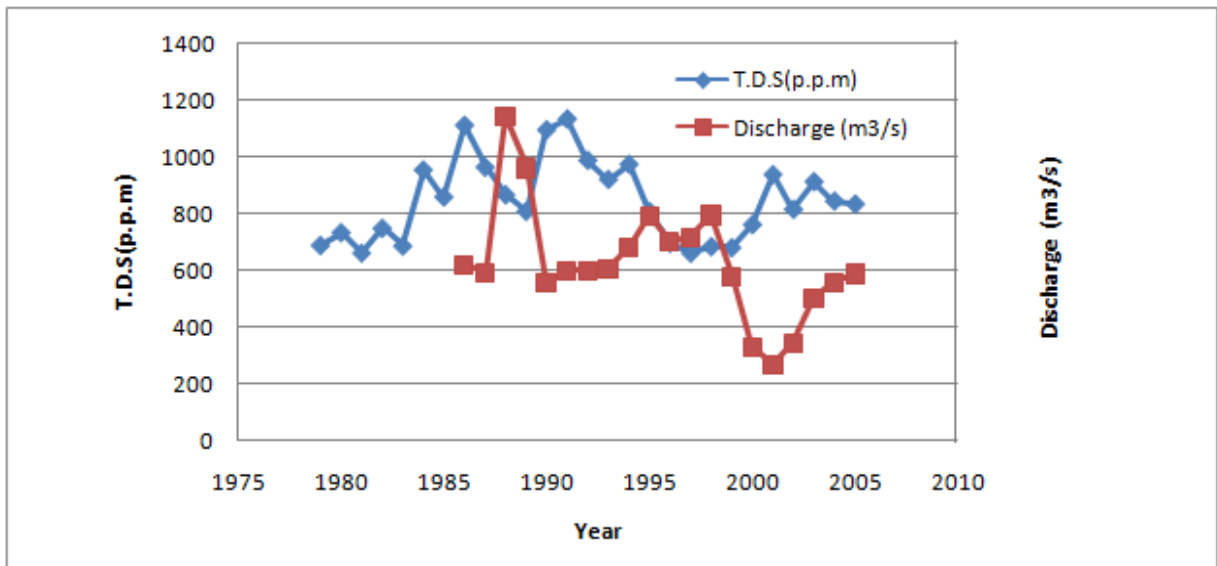
Fig.8 Salinity and discharge at Fallujah (Researchers)
