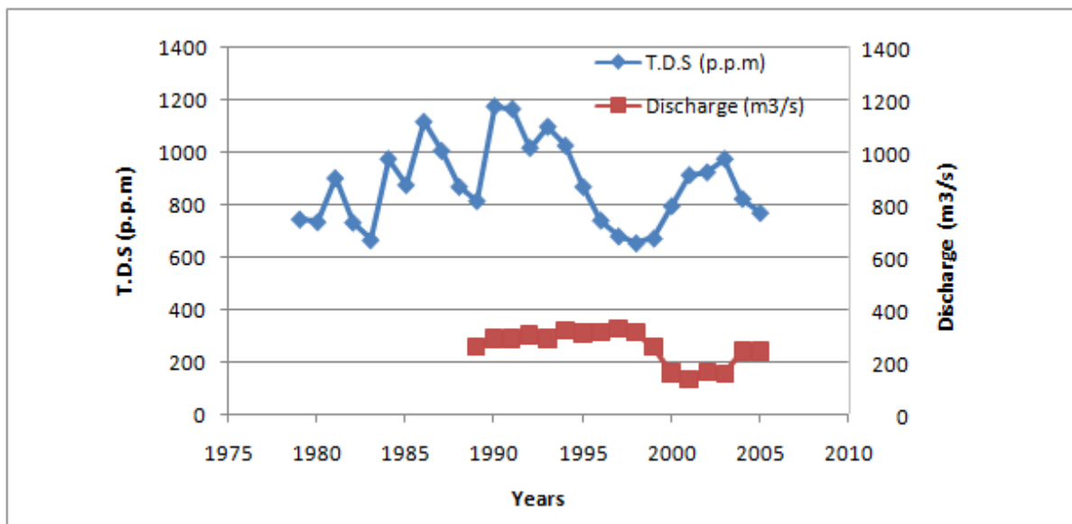
Fig. 9 Salinity and discharge at Hindya (Researchers)
