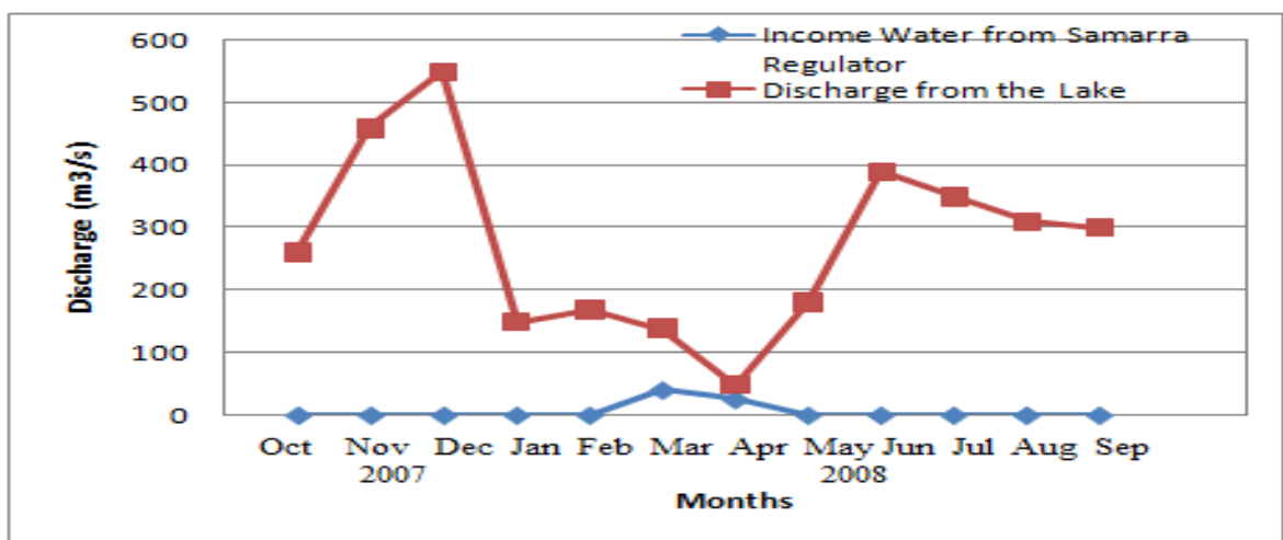
Fig.14 Income water from Samarra and discharge from Tharthar Lake (2006-2007) (Researchers)
