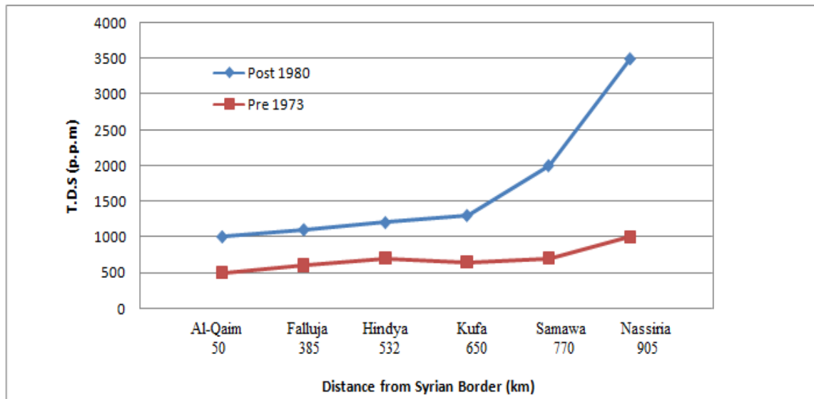
Fig. 5 Salinity along the Euphrates course prior to 1973 and after 1980 as extracted from the literature (Rahi, 2010)
