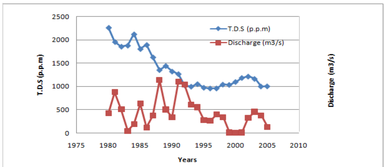
Fig. 12 Salinity and discharge from Tharthar lake to Euphrates River (Researchers)
