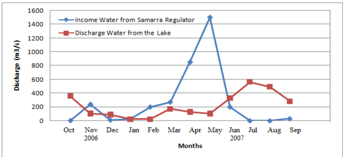
Fig.13 Income water from Samarra and discharge from Tharthar Lake (2006-2007) (Researchers)
