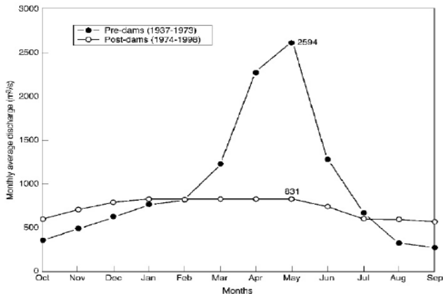
Fig. 3 Inflow of Euphrates River at Hit Pre. And Post dams Built. Source: UNEP (2001).
