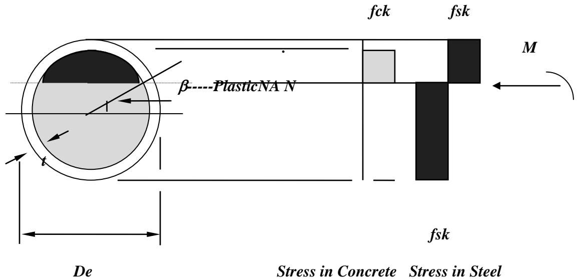
Fig 4 Stress Distribution in Concrete- Filled Circular Hollow Section at Muy.
