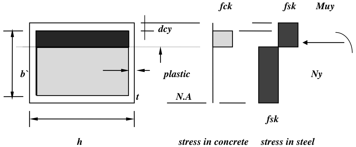
Fig 3 Stress Distribution in Concrete- Filled Rectangular Hollow section at M_{uy} .
