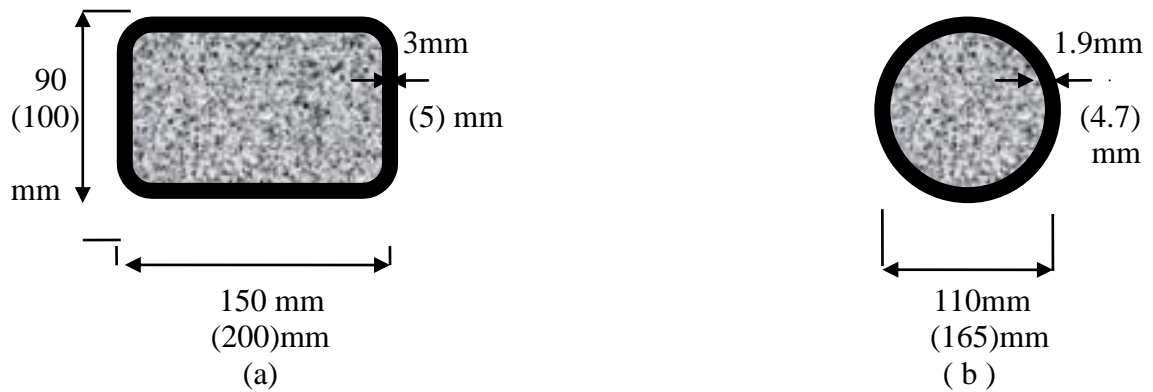
Fig. 1 Cross-Sectional Dimensions of Test Specimens: (a) Concrete-Filled RHS; (b) Concrete-Filled CHS.
